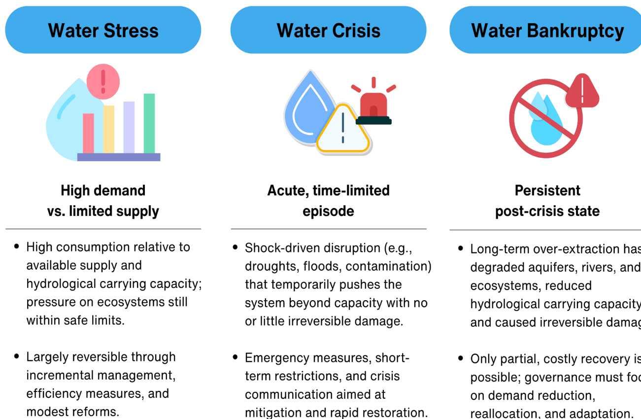
Figure 12. Three states of concern in human–water systems. The figure illustrates the major distinctions between water stress, water crisis, and water bankruptcy. These states reflect different levels of pressure on water resources and the underlying natural capital, requiring different responses by governments and stakeholders. Misidentifying the real state of the system can result in implementing ineffective or even wrong solutions. Figure adapted from Madani 6 .
