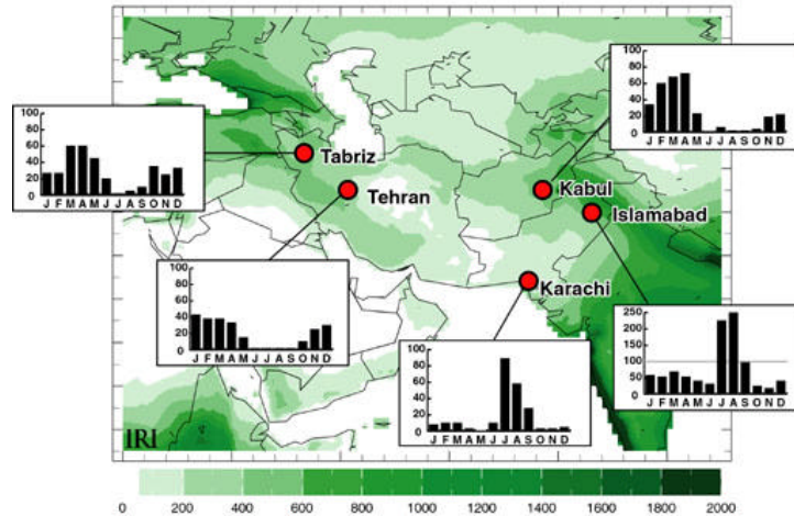
Figure 3 Regional rainfall patterns in Afghanistan and surrounding countries 12 .
