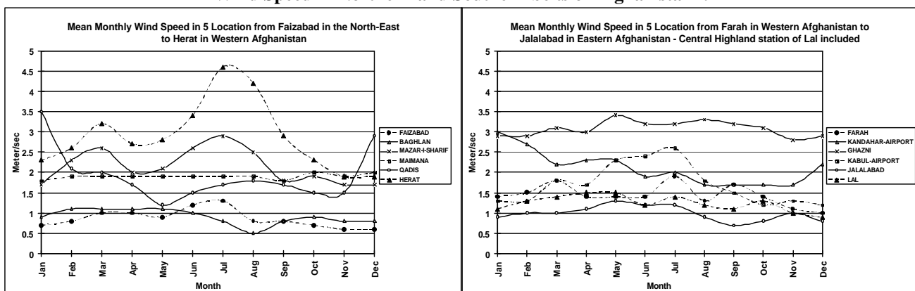
Graphs 1 and 2 Wind Speed in Northern and Southern belts of Afghanistan 11 .
