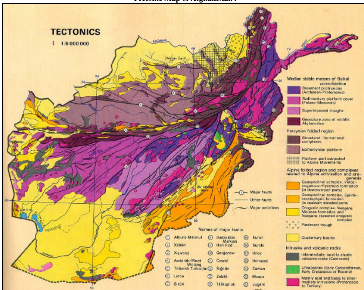
Figure 2 Tectonic Map of Afghanistan 7 .
