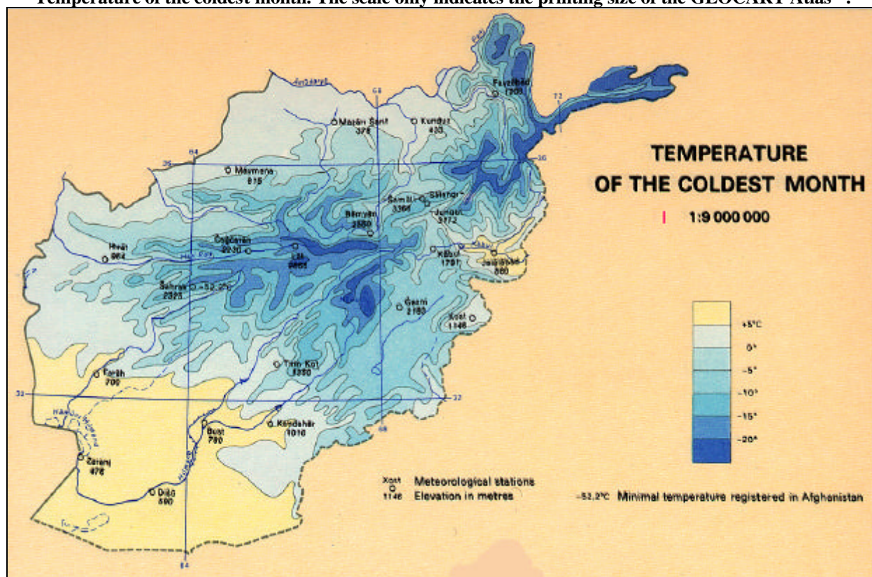
Figure 5 Temperature of the coldest month. The scale only indicates the printing size of the GEOCART Atlas 15 .
