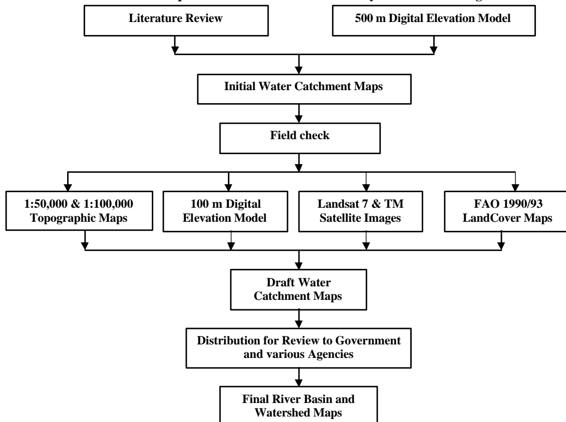
Figure 8 Flowchart on the process of the watershed boundary delineation for Afghanistan
