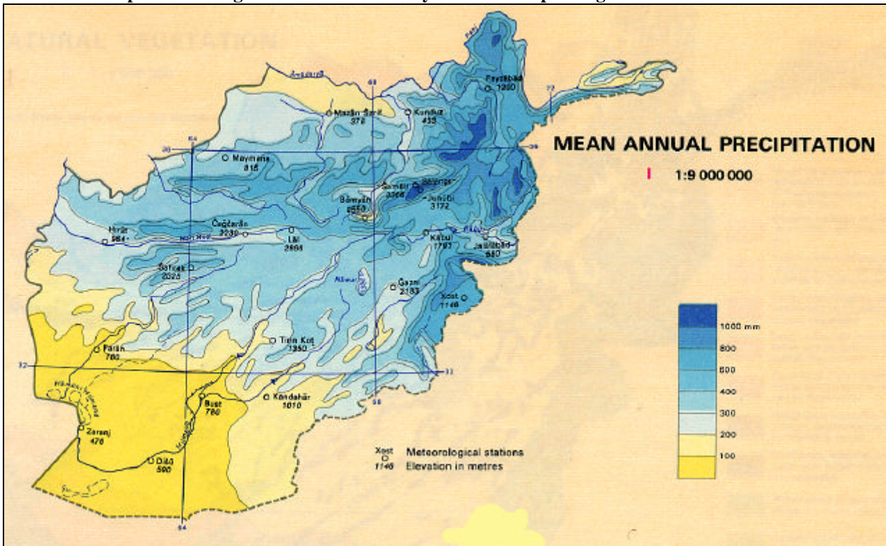
Figure 4 Annual Precipitation in Afghanistan. The scale only indicates the printing size of the GEOCART Atlas 13 .
