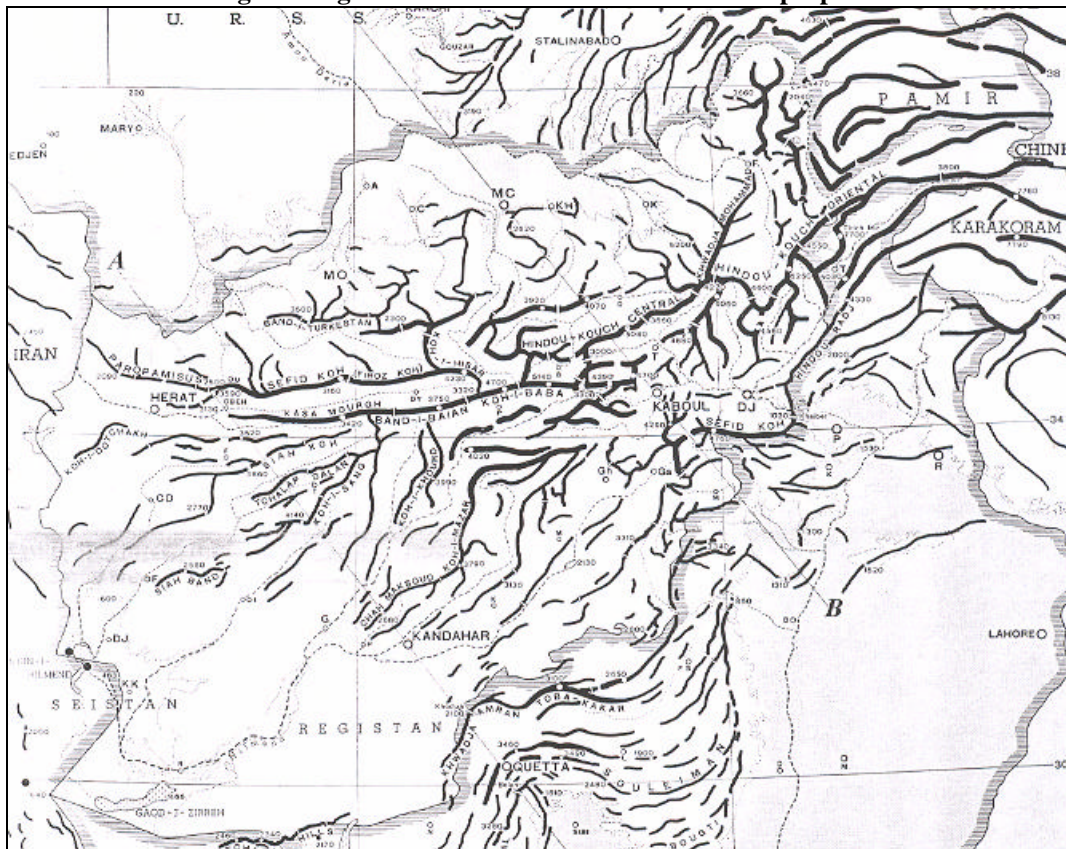
Figure 1 Main Mountain ranges in Afghanistan. The thickness of the lines is proportional to elevation 4 .
